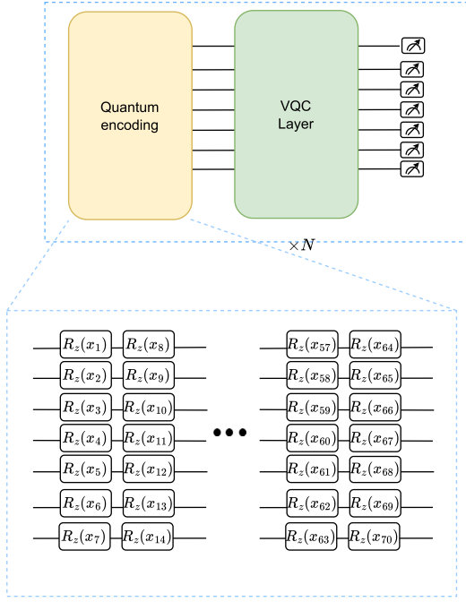
Fig. 3. Structure of the quantum encoding layer in QMLSC, demonstrated using an input of size 10 \times 7 .
