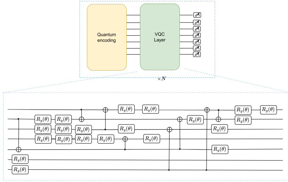
Fig. 5. The structure of the variational quantum circuit layer in QMLSC (exemplified by the model implemented on the MELD dataset).
