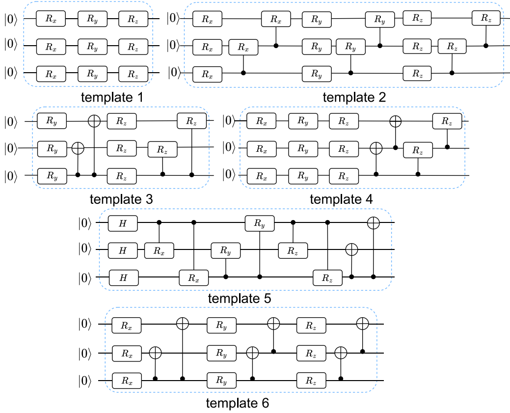
Fig. 7. The template set consists of circuits inspired by or derived from previous research, with dashed boxes denoting individual circuit layers that can be repeated.
